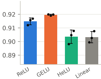
Fashion-MNIST CNN
