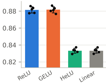
Fashion-MNIST MLP
