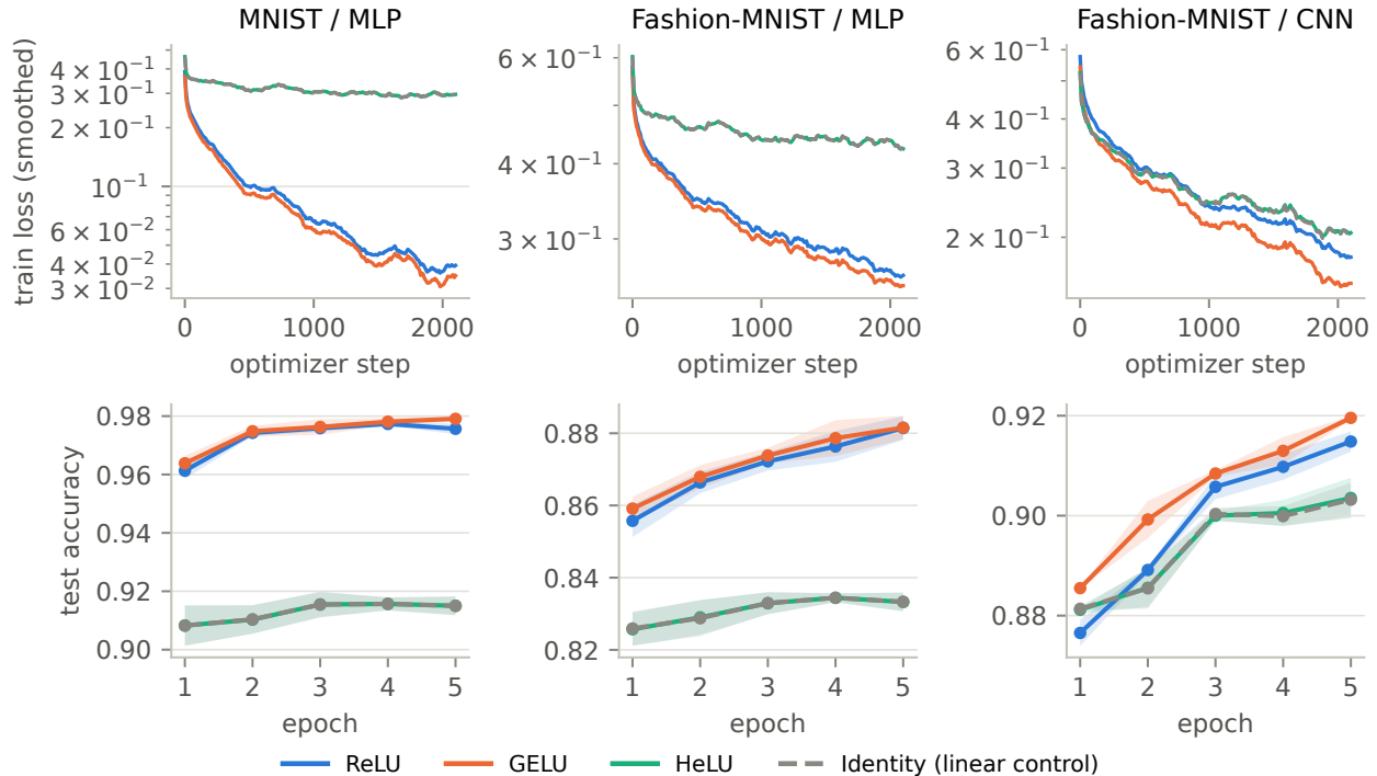
Figure 4: Training dynamics on the image benchmarks (E4, E5). Top: training loss, averaged over seeds after a 25-step moving average. Bottom: test accuracy after each epoch, shaded bands are \pm 1 sd over seeds.
