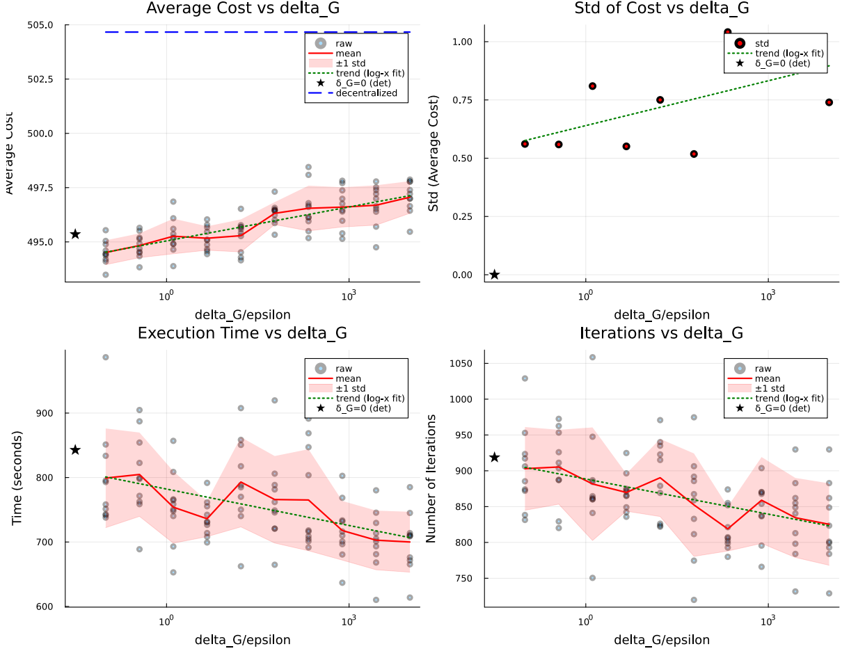
Figure 4: Sweep over \delta_G for 10 buildings (day 37, 10 repeats per point). Top-left : average cost per building (dashed = decentralised baseline). Top-right : std of cost across repeats. Bottom-left : execution time. Bottom-right : ADMM iterations per MPC step. The \delta_G = 0 anchor (star) is deterministic (std=0).
