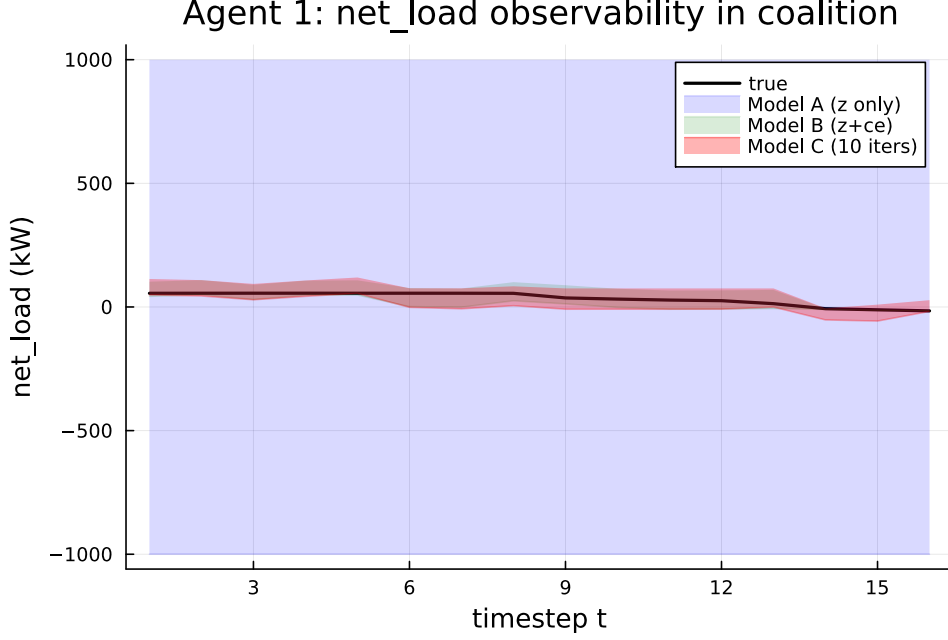
Figure 3: Per-timestep d bounds for agent 1 in the 2-agent coalition. Model A (blue) is unbounded; Model B (green) is tightest; Model C with 10 iterations (red) is intermediate. The true d (black) lies within all bounds.
