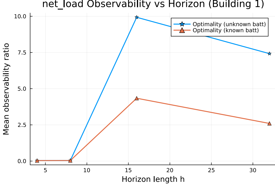
Figure 2: d observability ratio vs. horizon length for building 1. Short horizons ( h \leq 8 ) have no price variation, so the battery is unused and d = z^* (trivially observable). At h = 16 , the price change activates the battery and observability degrades sharply. Longer horizons ( h = 32 ) provide more data, slightly improving observability.
