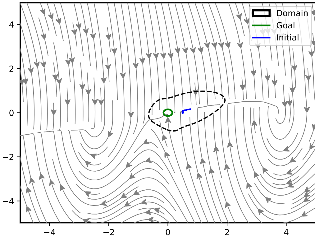
Phase Plane
