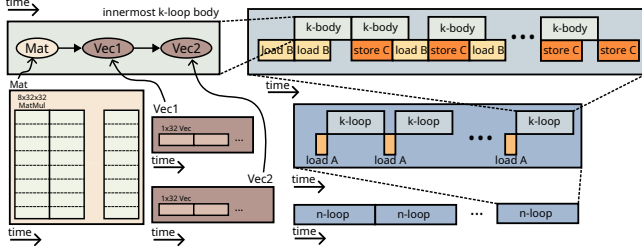
Figure 4: Pipelined execution of a matrix multiplication.
