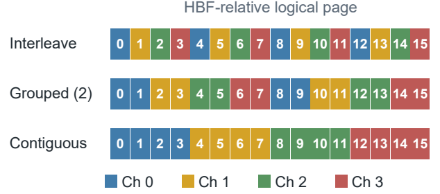
Figure 7: Channel assignments under three placement policies. Interleave rotates channels after each page; grouped placement rotates after every two pages. Contiguous placement assigns consecutive active pages to each channel.
