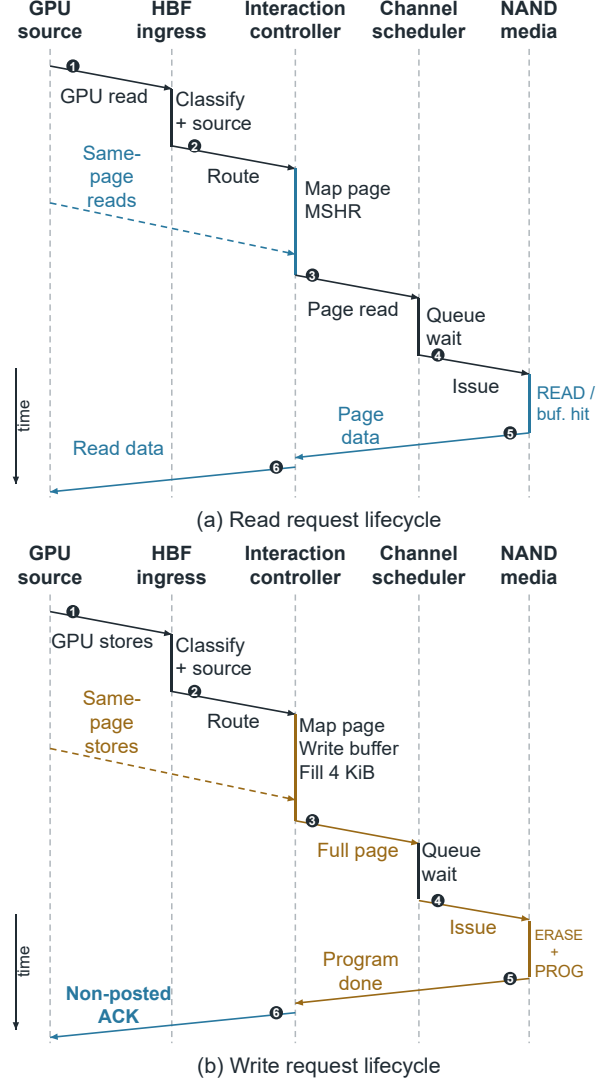
Figure 4: Request lifecycle through HBF-Sim. A GPU read or write request enters the interaction controller, is mapped to one stack and channel, and follows page tracking, queueing, and NAND service before read data or write status returns to the source GPU partition.
