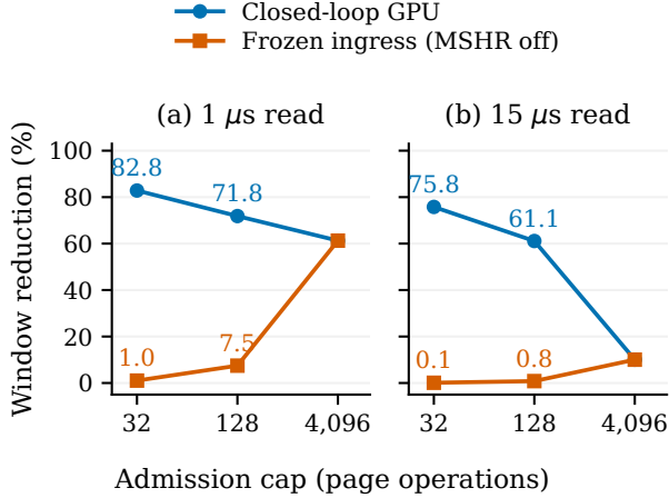
Figure 5: Frozen ingress understates MSHR benefits under admission pressure. HBF completion-window reduction relative to merging disabled, using 16 pages and 32 entries per page. Replay fixes the baseline’s ingress times.
