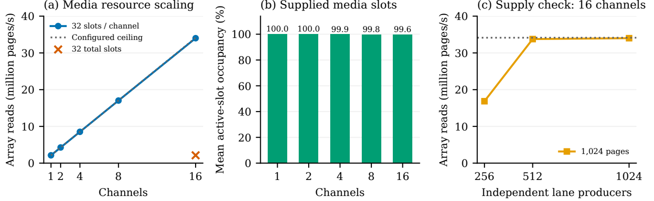
Figure 6: Media scaling with 32 subarrays and active slots per channel at 15 \mu s reads. Throughput counts array pages, not GPU payload bytes. Occupancy and producer-count controls check saturation.
