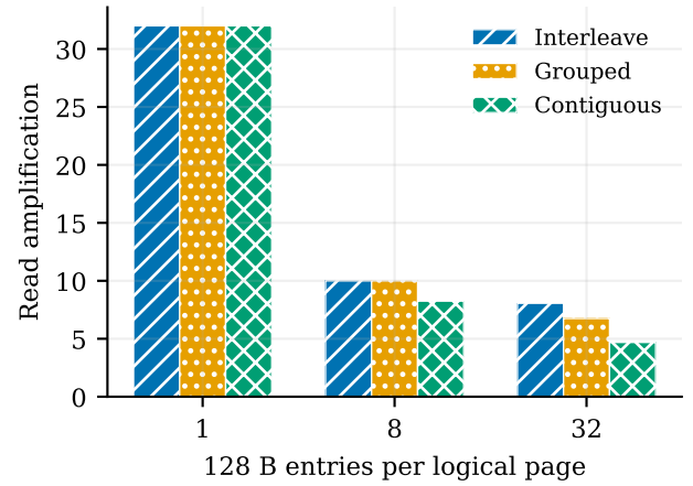
Figure 8: Page-service amplification under shortened timing ( t_R = 20 DRAM ticks). At 32 entries per page, contiguous placement reduces page-service amplification by 41.9% relative to interleave. Page services include NAND page-buffer hits.
