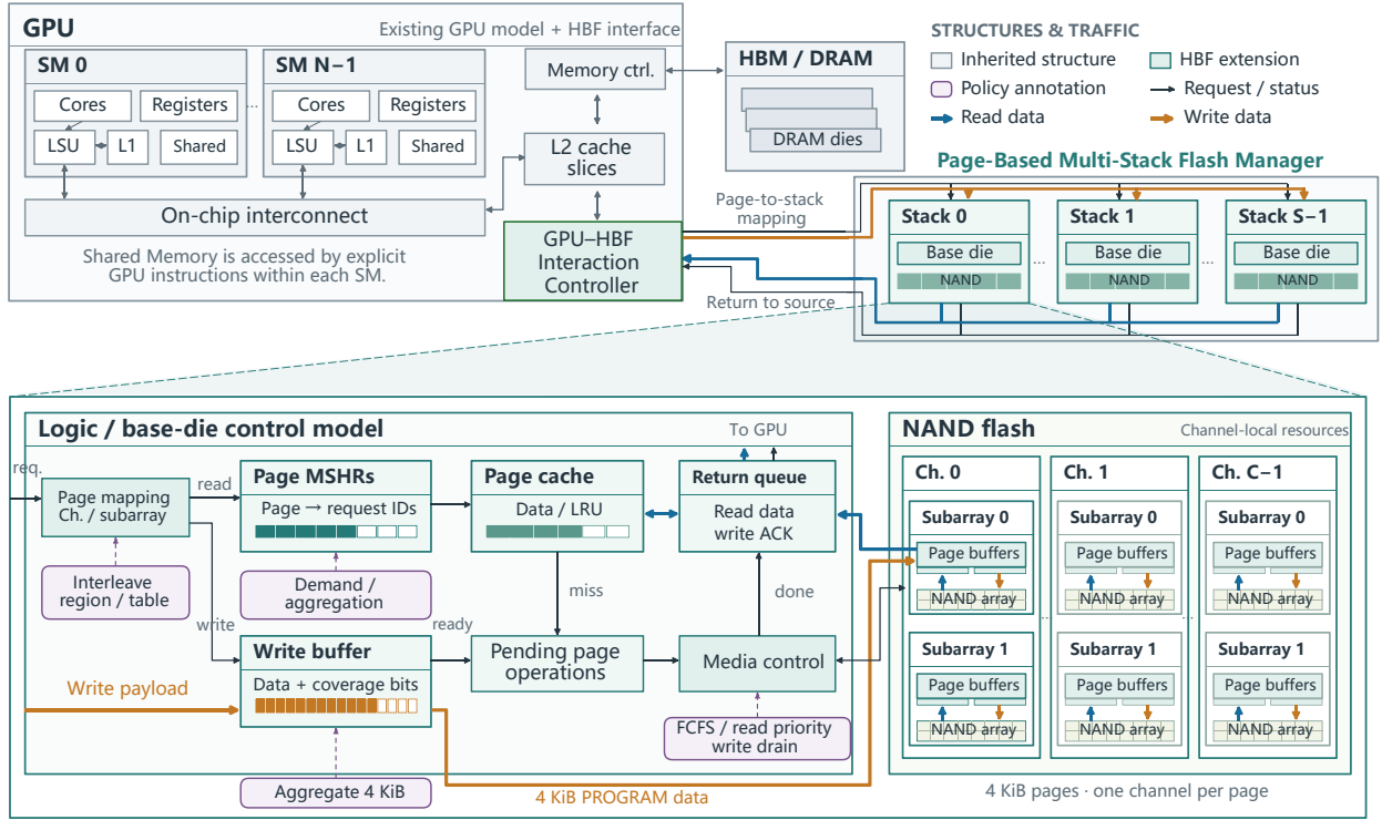
Figure 2: HBF-Sim architecture. The upper part shows GPU memory paths and independent HBF stacks. The lower part expands one stack into its control structures and channel-owned NAND resources. Rectangles denote modeled structures, while the figure’s policy annotations identify configurable methods. Thin arrows carry requests or control/status. Thick blue and orange arrows carry read and write data.
