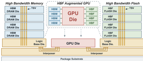
Figure 1: Overview of an HBF-augmented GPU package. The inset shows HBM and HBF stacks beside the GPU; cross-section shows DRAM and NAND dies, TSVs, microbumps, logic/base dies, the interposer, and package substrate.
