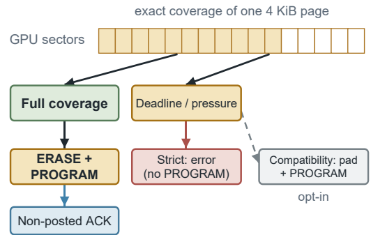
Figure 3: Page-based write aggregation. Incomplete pages trigger an error on flush or are padded in compatibility mode. The GPU receives a completion response only after the full page is written to NAND.
