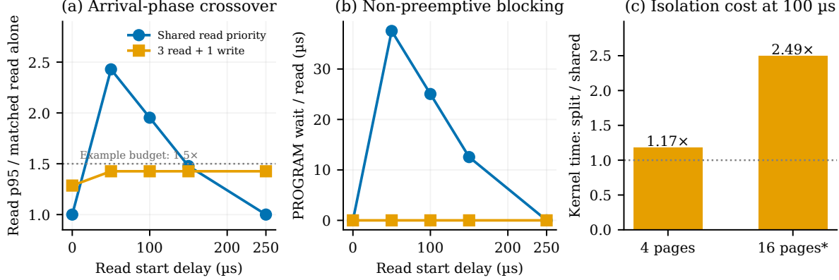
Figure 9: Read protection depends on arrival phase and resource allocation. (a) Read p95 is normalized to a matched read-only run. (b) Average time per read spent queued while its target subarray is executing PROGRAM. The average includes all read requests and is not added to kernel time. (c) Isolation changes whole-kernel time. The starred 16-page comparison uses a matched, extended 400 \mu s assembly deadline. The original isolated configuration is infeasible under the shorter deadline. The 1.5 \times line is an illustrative budget.
