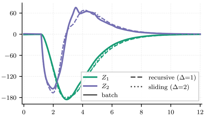
Delays and applied prediction horizon
