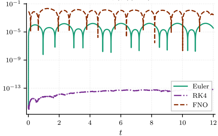
Residual \phi(\hat{\psi}(t) + t) - t
