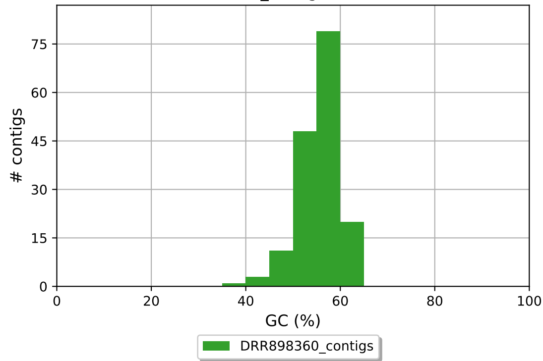
DRR898360_contigs GC content
