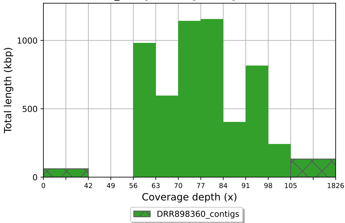
DRR898360_contigs coverage histogram (bin size: 7x)
