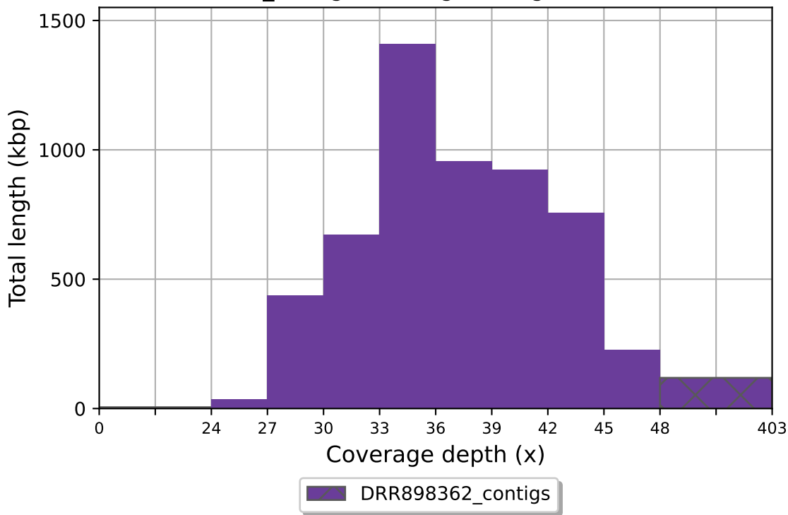
DRR898362_contigs coverage histogram (bin size: 3x)
