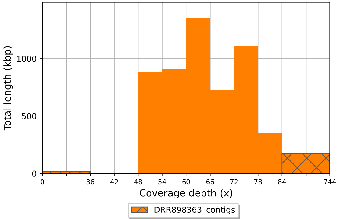
DRR898363_contigs coverage histogram (bin size: 6x)
