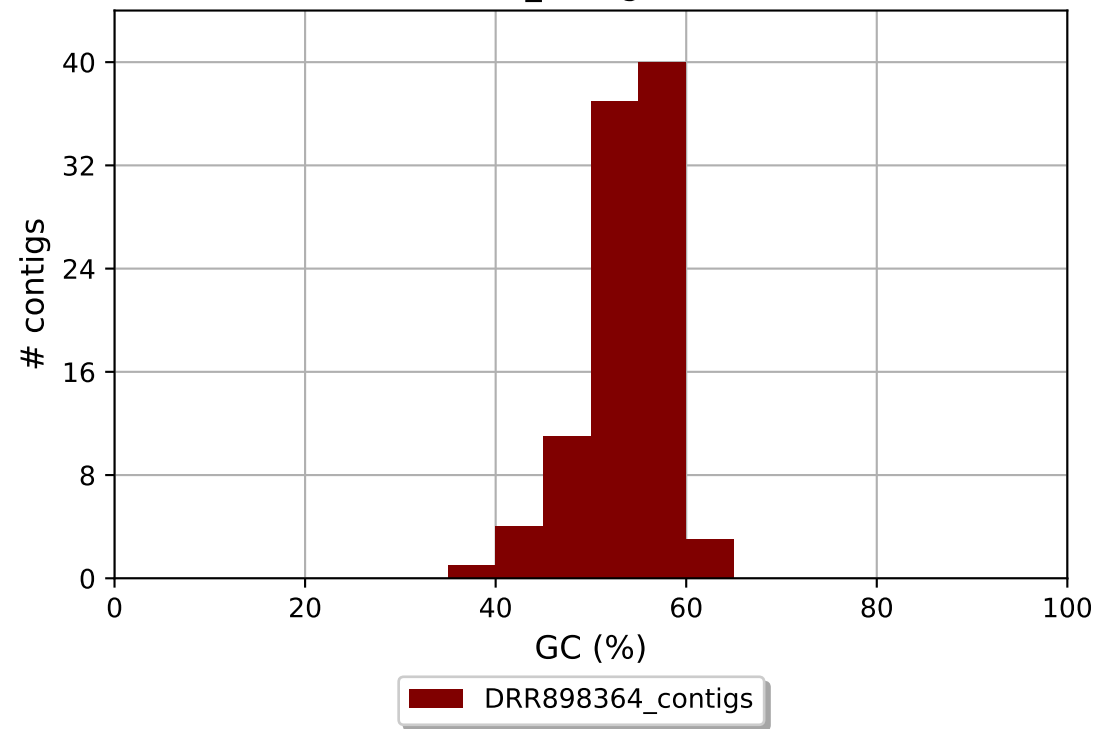
DRR898364_contigs GC content
