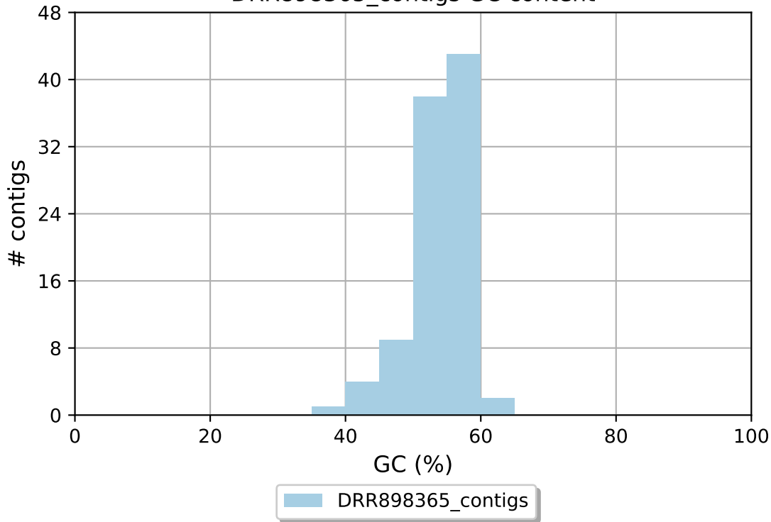
DRR898365_contigs GC content
