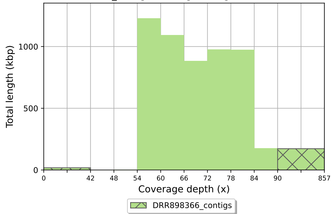
DRR898366_contigs coverage histogram (bin size: 6x)
