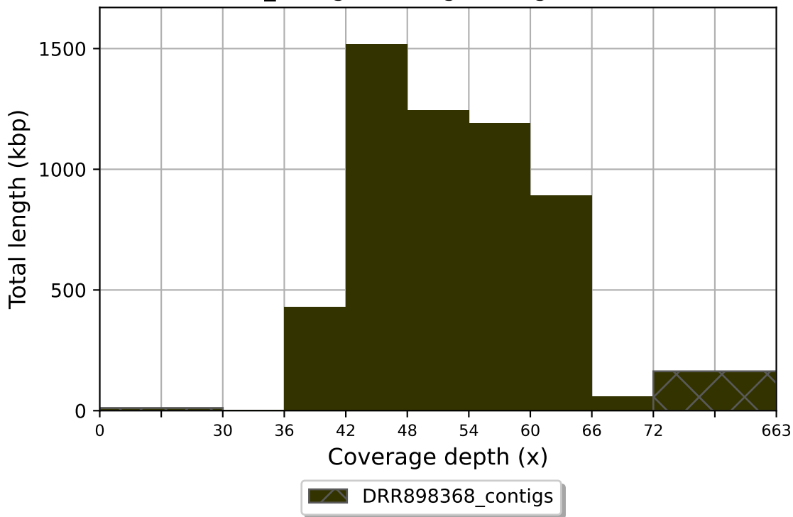
DRR898368_contigs coverage histogram (bin size: 6x)
