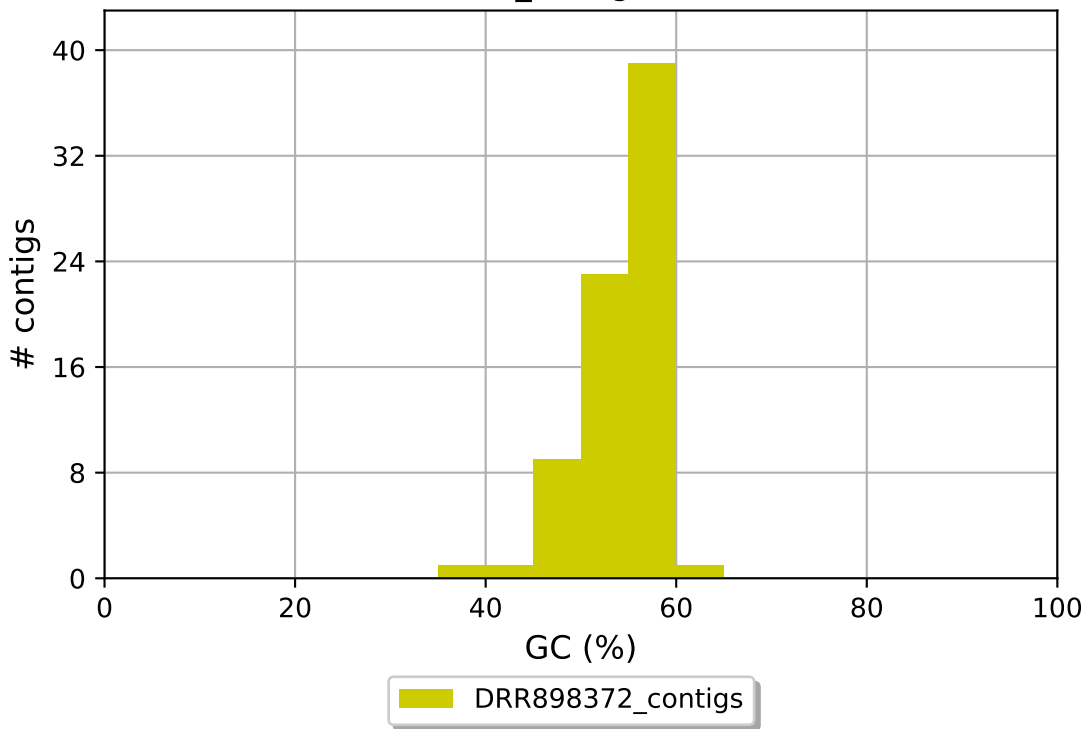
DRR898372_contigs GC content
