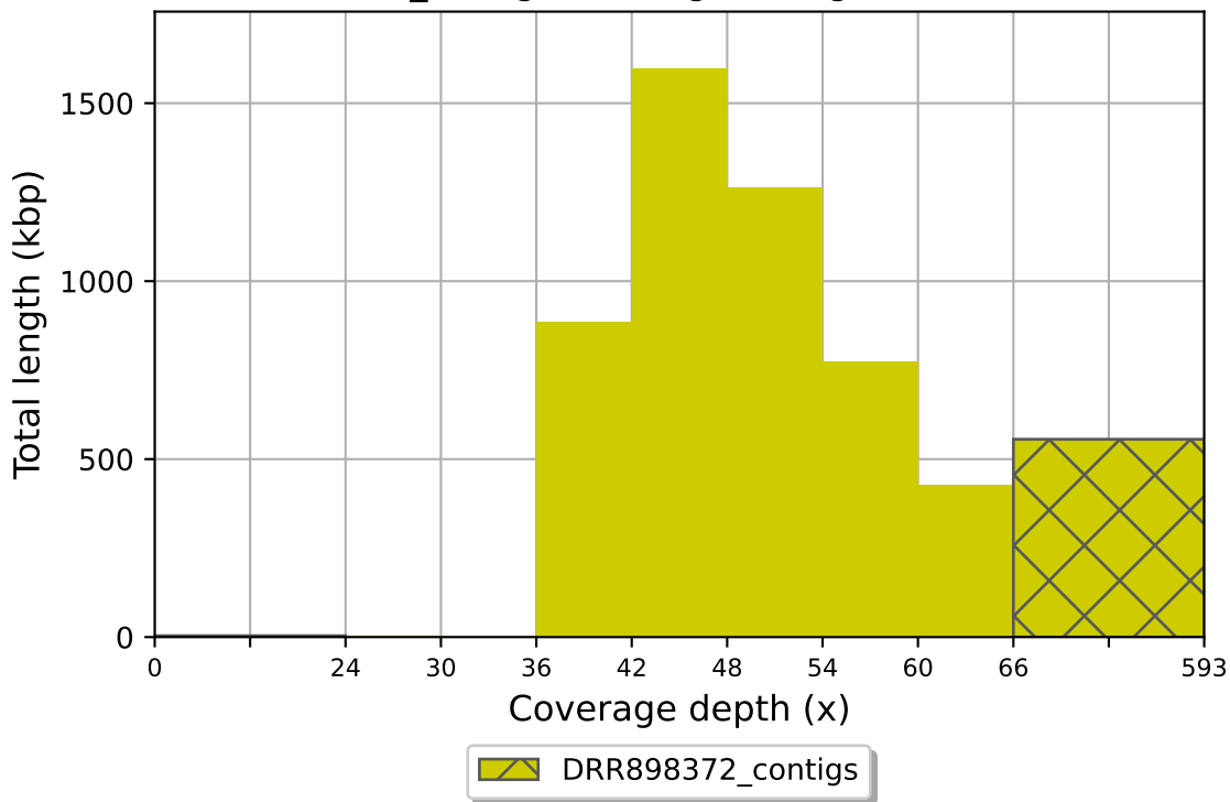
DRR898372_contigs coverage histogram (bin size: 6x)
