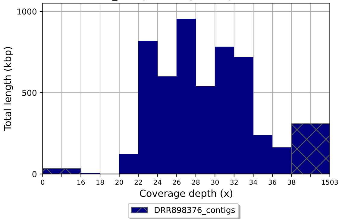
DRR898376_contigs coverage histogram (bin size: 2x)
