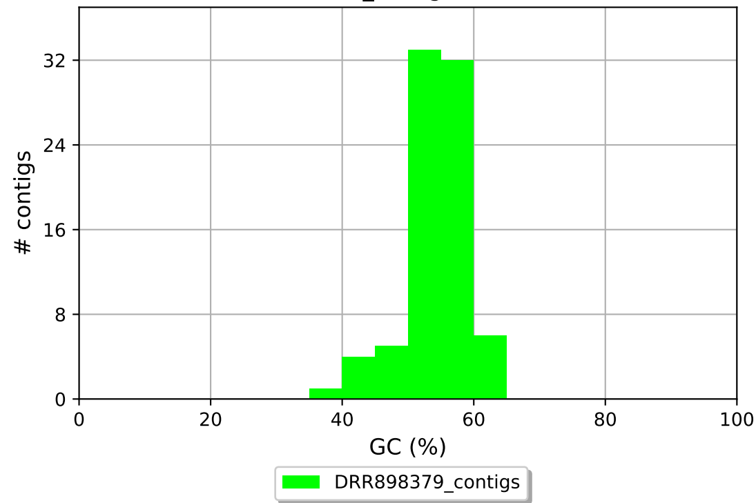
DRR898379_contigs GC content
