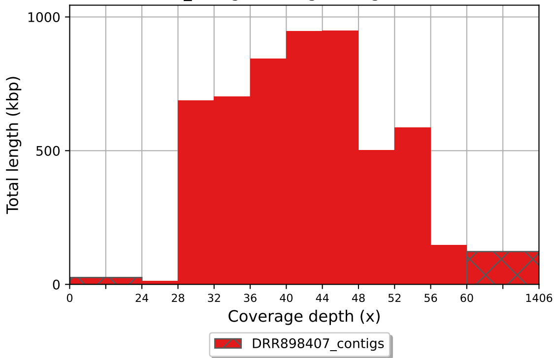
DRR898407_contigs coverage histogram (bin size: 4x)
