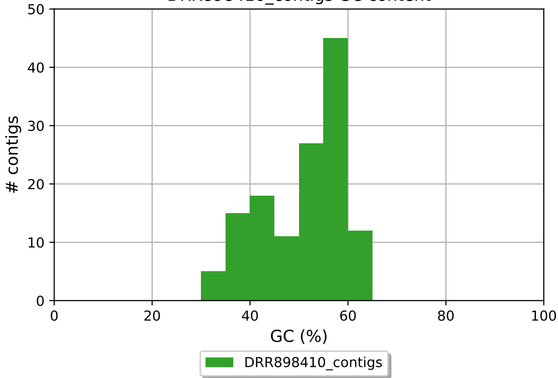
DRR898410_contigs GC content
