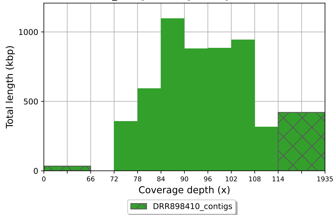
DRR898410_contigs coverage histogram (bin size: 6x)
