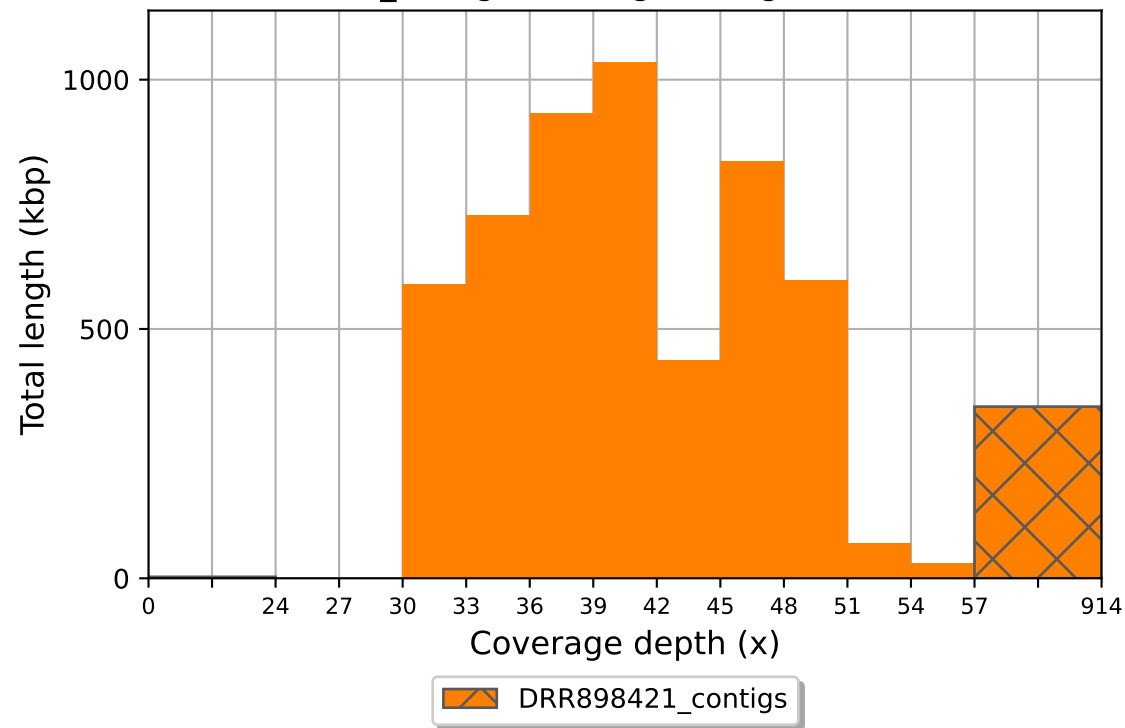
DRR898421_contigs coverage histogram (bin size: 3x)
