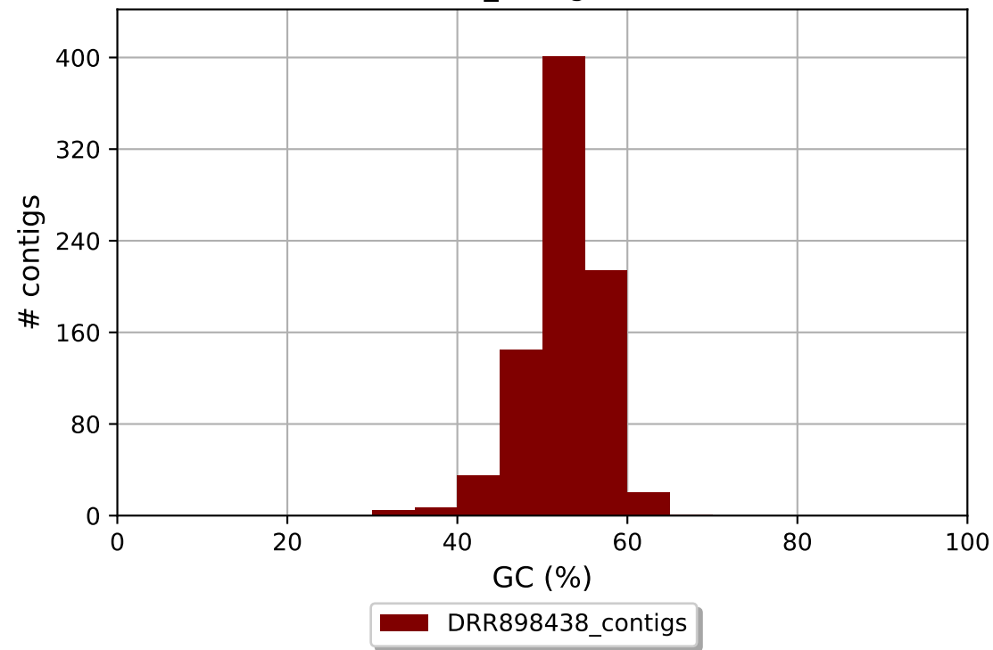
DRR898438_contigs GC content
