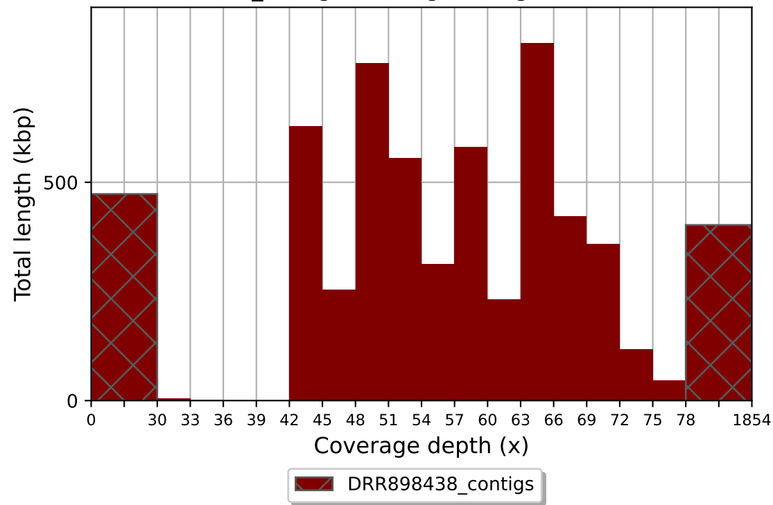
DRR898438_contigs coverage histogram (bin size: 3x)
