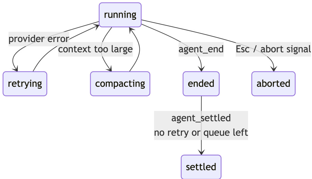
Figure 7.4: Run lifecycle. Retries and compaction resume the run; agent_end fires when the loop stops, agent_settled when no automatic continuation remains.
