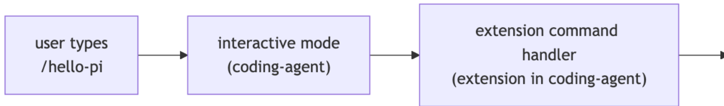
Figure 6.2: The /hello-pi trace. Each arrow crosses a package boundary; only the last one leaves the process.
