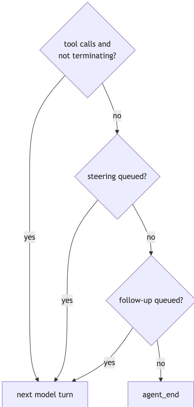
Figure 4.3: After a toolResult is appended, the loop decides what happens next. Queued steering beats follow-up; an empty loop emits agent_end.
