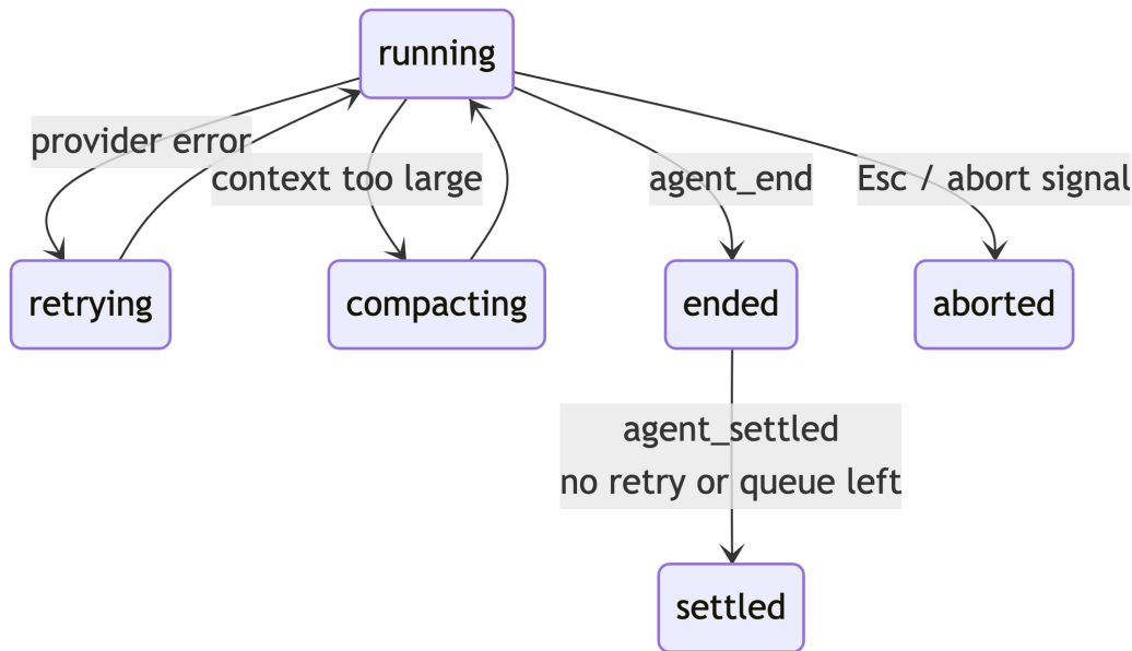
Figure 4.4: Run lifecycle. Retries and compaction resume the run; agent_end fires when the loop stops, agent_settled when no automatic continuation remains.
