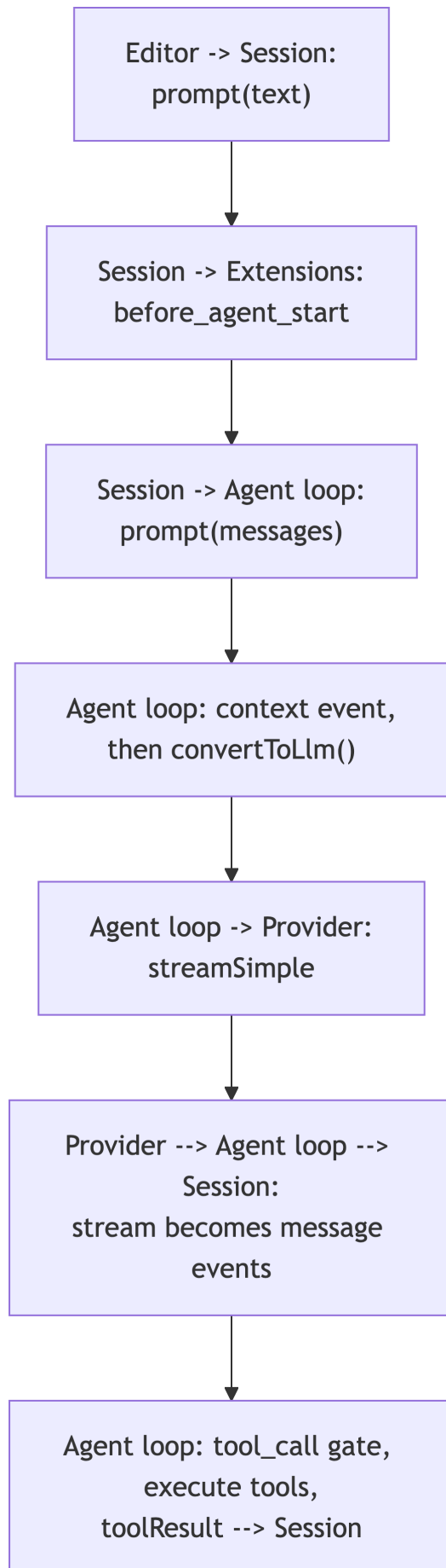
Figure 4.2: One turn across stages 3-6: turn construction, context conversion, provider dispatch, and
