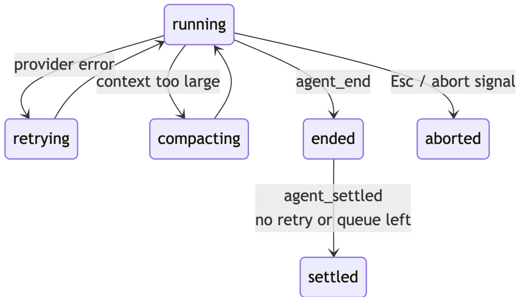
Figure 6.4: Run lifecycle. Retries and compaction resume the run; agent_end fires when the loop stops, agent_settled when no automatic continuation remains.
