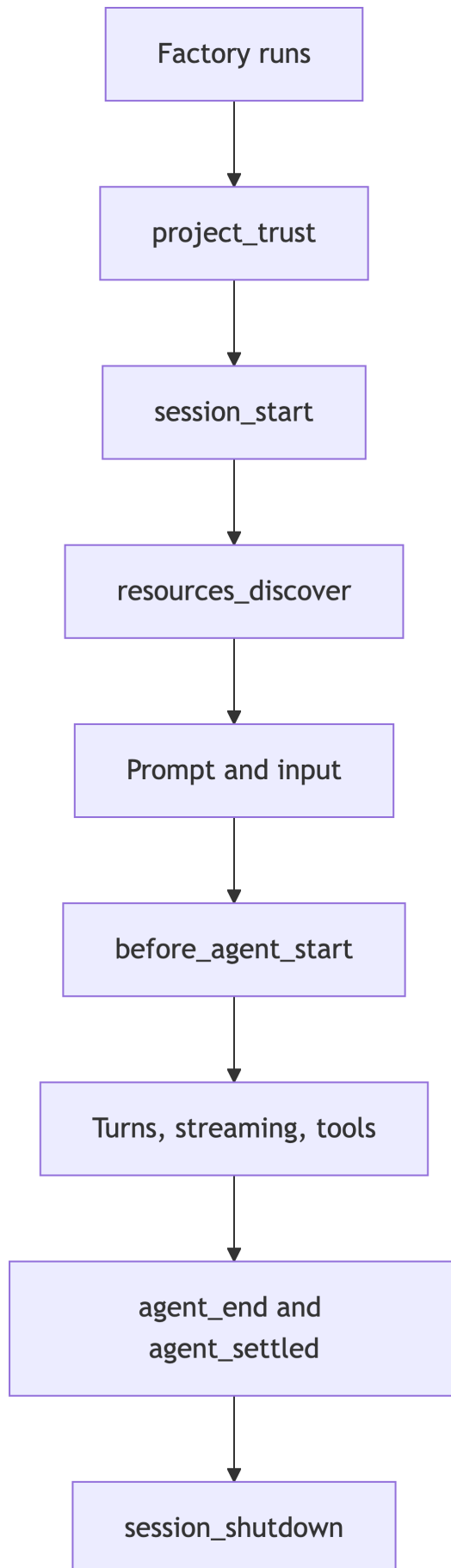
Figure 7.1: Representative extension event flow (not exhaustive).
