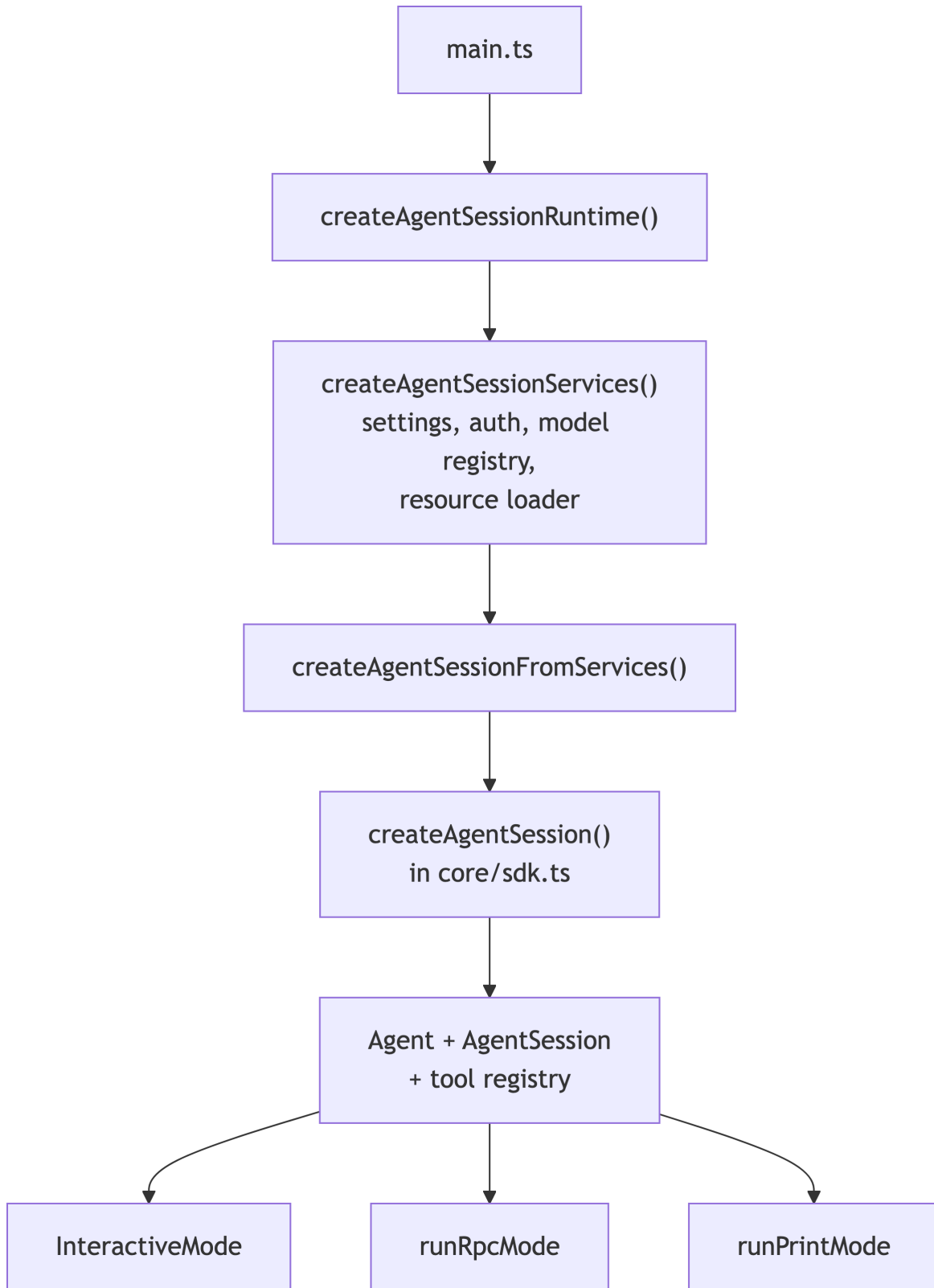
Figure 5.2: Startup construction. Services are built first, the session wraps an Agent around them, then one of the three run modes takes over.
