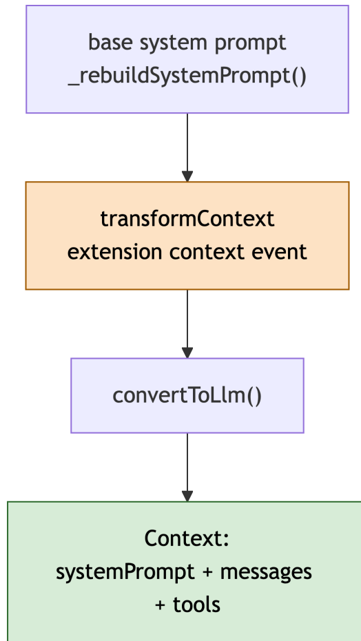
Figure 7.2: Stage 4’s three construction boundaries. The extension context event (amber) sits between base system-prompt assembly and provider conversion; the output is a Context with exactly systemPrompt, messages, and tools.
