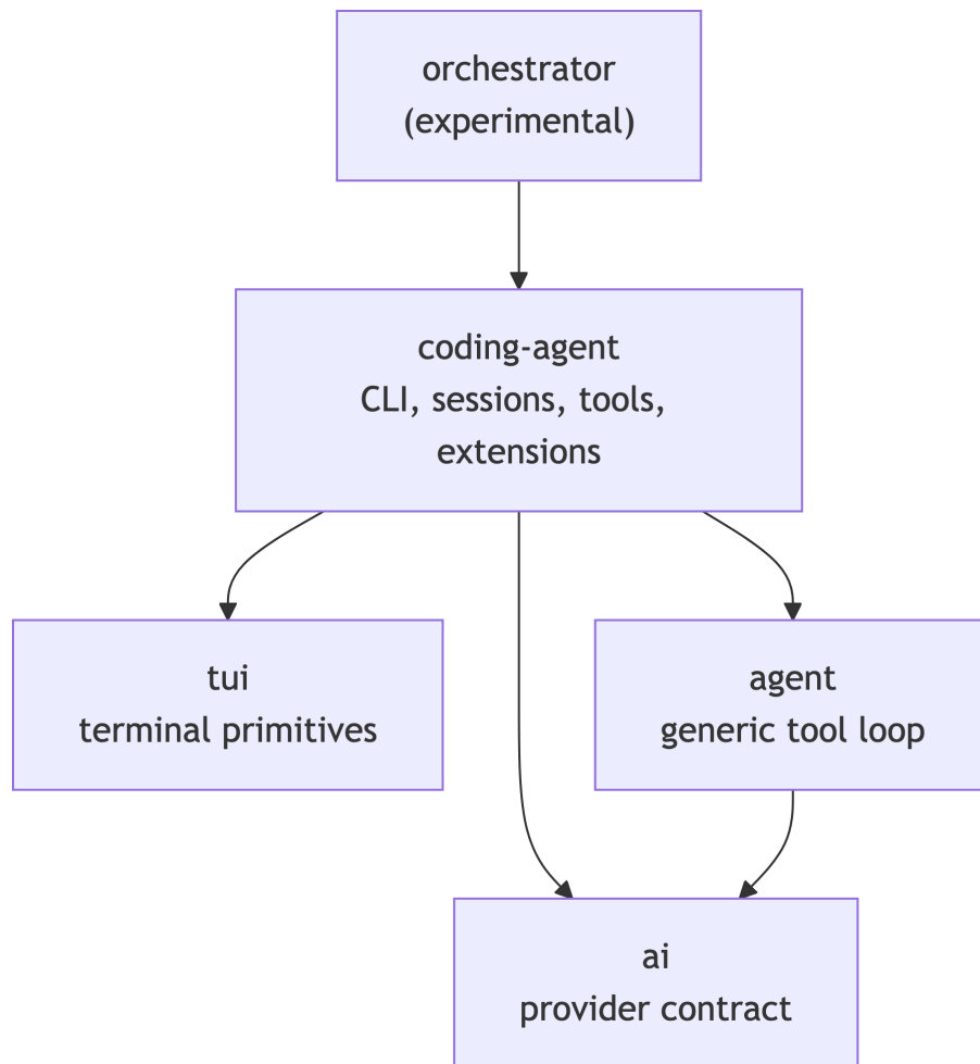
Figure 6.1: The package map. An arrow points from a package to the package it imports; lower layers never import higher ones.
