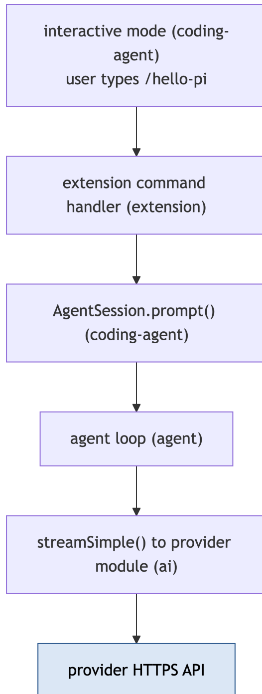
Figure 6.2: The /hello-pi trace. Each arrow crosses a package boundary; only the last one leaves the process.
