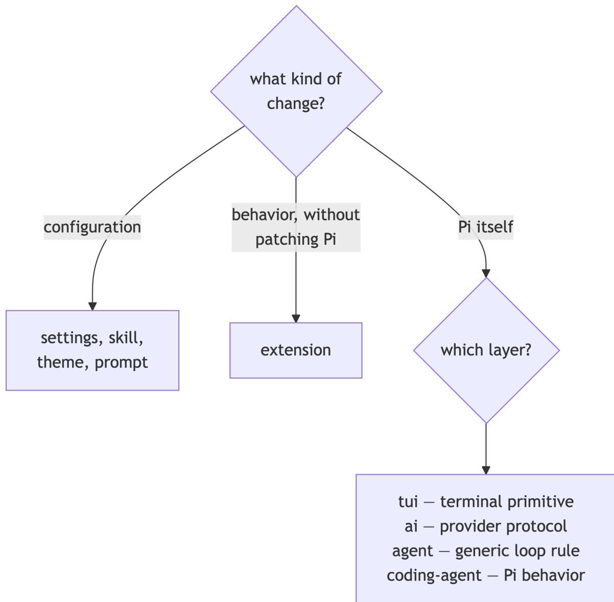
Figure 6.4: Where a change belongs. Code changes go to the owning layer; everything else is a resource or an extension.
