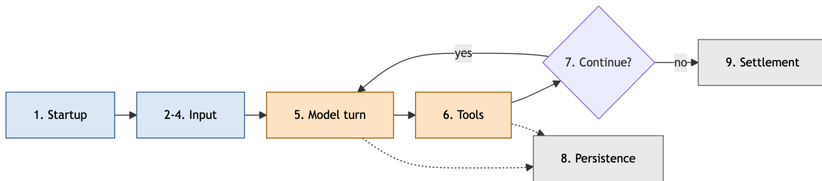
Figure 7.2: The complete prompt path. Startup loads and trusts extensions; input and interception build the run; each model turn assembles context, calls the provider, and streams; tools are validated, gated, and executed; persistence records finalized work throughout; settlement closes the run.
