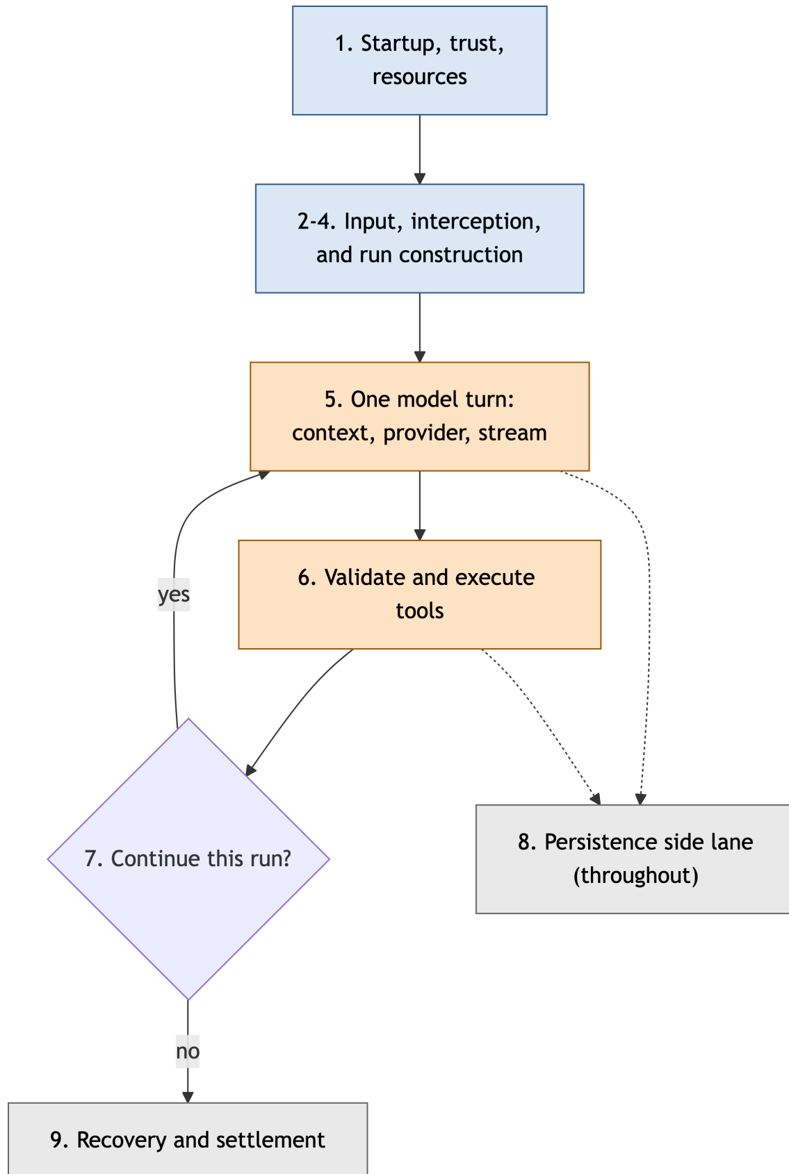
Figure 7.1: The complete prompt path. Startup precedes the loop; prompt and tool assembly precede the repeated provider/tool cycle; persistence is a side lane; settlement closes the run.
