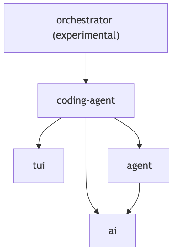
Figure 3.1: Runtime dependency direction. An arrow points from a package to the package it imports; lower layers never import higher ones.
