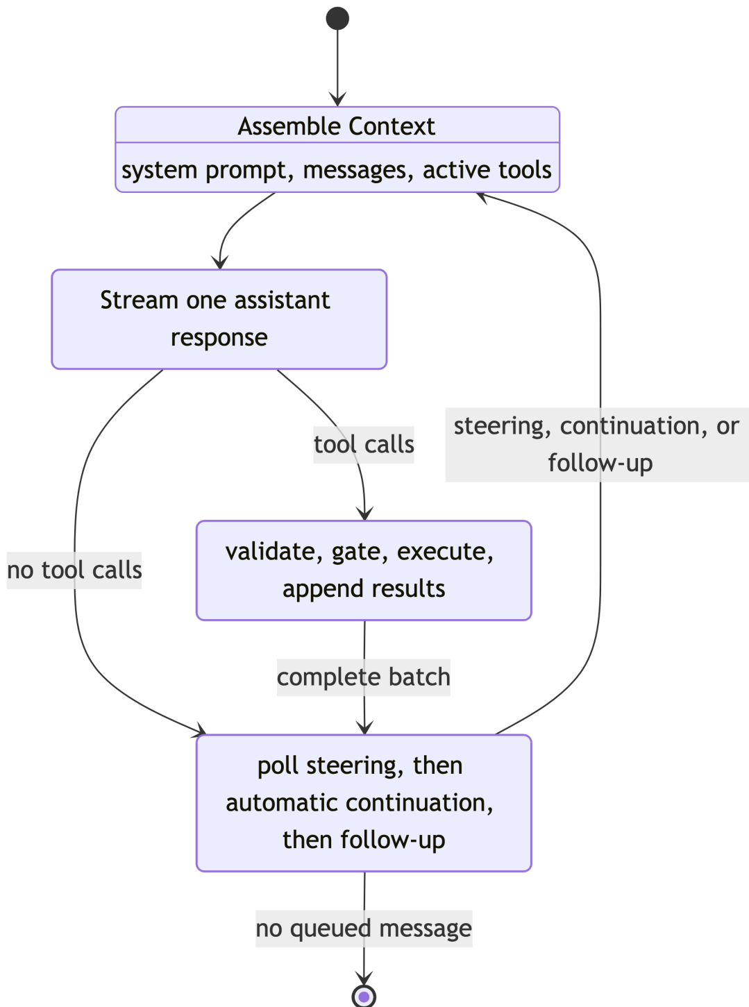
Figure 7.1: The model-facing loop. Tool schemas and tool guidance have different roles: schemas are sent in Context; guidance helps construct the system prompt.
