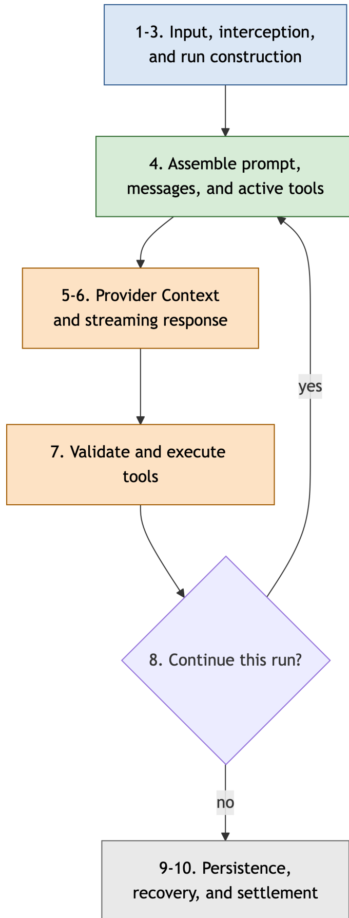
Figure 7.3: The complete interactive prompt path. Prompt and tool assembly precede the repeated provider/tool cycle; persistence and session settlement happen after the low-level loop ends.
