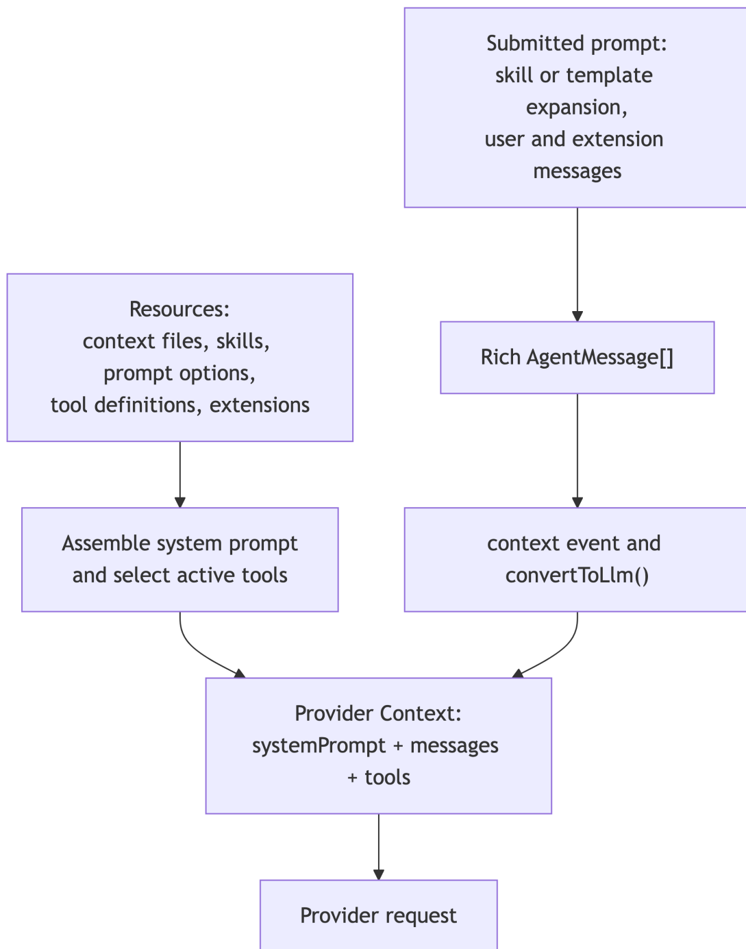
Figure 7.2: Model-context assembly. Resource discovery and input expansion happen before a run; messages are transformed and converted before every provider request.
