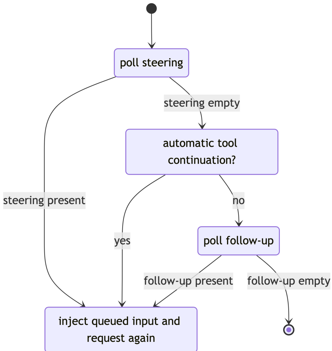
Figure 7.7: The queue boundary after a turn. Steering is polled before automatic tool continuation; follow-up is polled only after both are exhausted.
