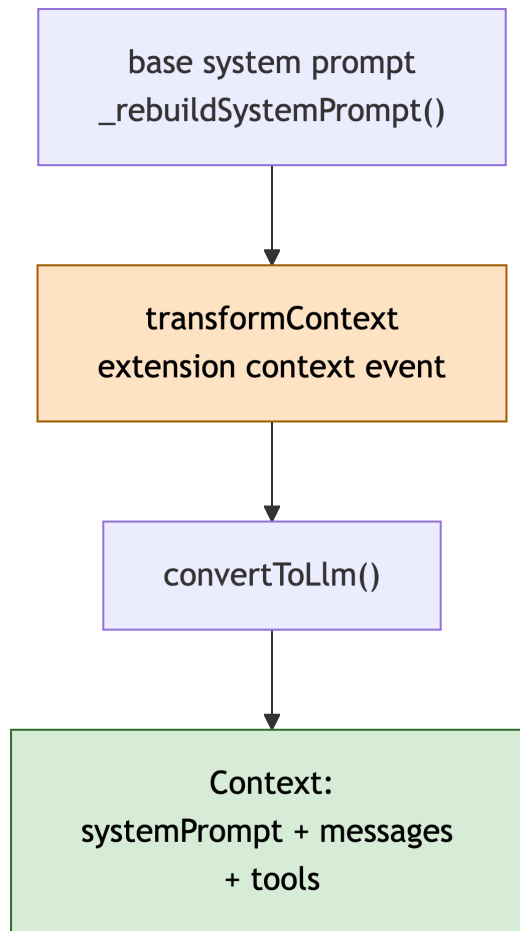
Figure 7.5: Stage 4's three construction boundaries. The extension context event (amber) sits between base system-prompt assembly and provider conversion; the output is a Context with exactly systemPrompt, messages, and tools.
