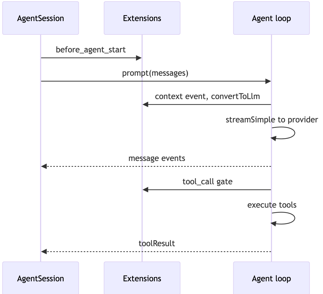
Figure 7.6: One turn across stages 3-6: turn construction, context conversion, provider dispatch, and the event stream back to the session. The turn begins when the editor calls AgentSession.prompt(text) .
