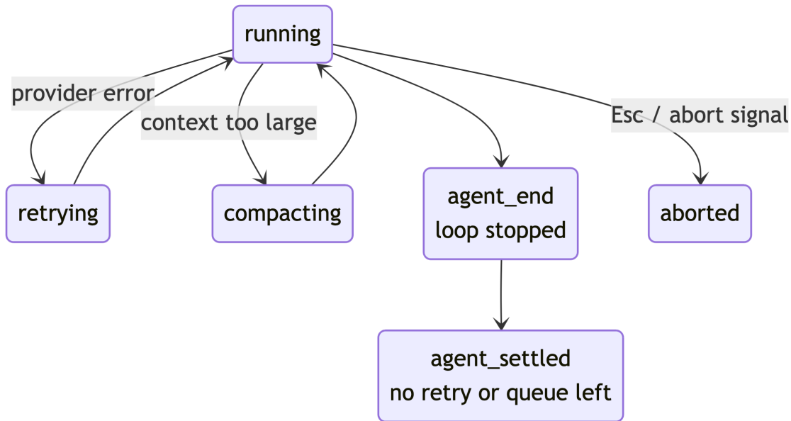
Figure 7.8: Run lifecycle. Retries and compaction resume the run; agent_end fires when the loop stops, agent_settled when no automatic continuation remains.
