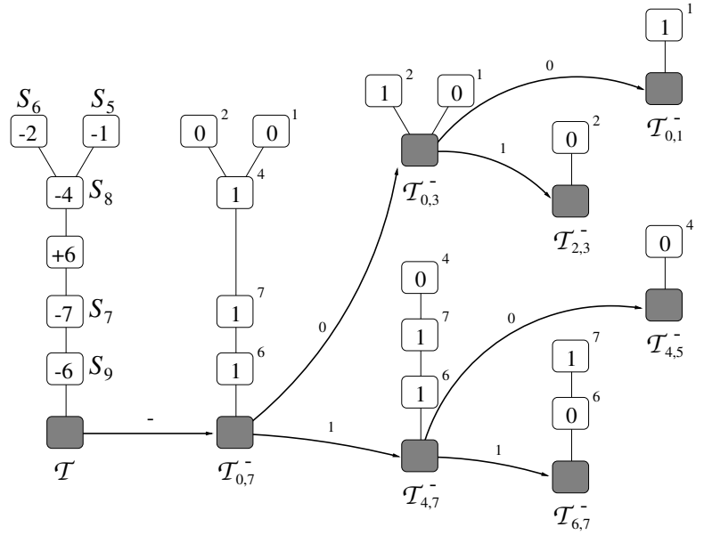
Figure 4.3: Hierarchical extraction of one indel-tree hierarchy, reproduced from Ggie, He, and Navarro [9]. The diagram shows the source example \mathcal{T}^- = \mathcal{T}_{0,7}^- obtained from the indel tree rooted at v(U) of Figure 4.2 (drawn upside down). The source figure pads the example to the range [0..7] , while the construction in this thesis uses [1..u] . At each intermediate range [a..b] , the 0/1-labelled tree \mathcal{T}_{a,b}^- extracts to \mathcal{T}_{a,m}^- on label 0 and to \mathcal{T}_{m+1,b}^- on label 1, following the bold rightward arrows. The same construction yields \mathcal{T}^+ on insertion marks. The coordinated descent of this subsection tracks images v^+ and v^- in two parallel instances of this structure.
