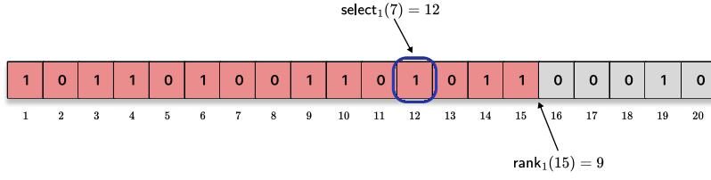
Figure 2.1: A bitvector B[1..20] . The prefix B[1..15] (shaded red) contains nine ones, so \text{rank}_1(B, 15) = 9 . The seventh one (circled blue) lies at position 12, so \text{select}_1(B, 7) = 12 .
