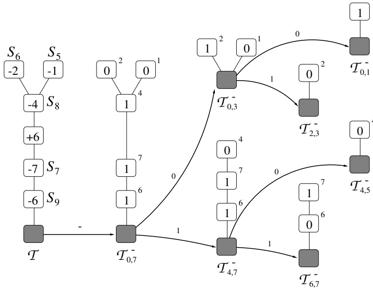
Figure 4.3: Hierarchical extraction of one indel-tree hierarchy, reproduced from Gaggie, He, and Navarro [9]. The diagram shows GHN’s worked example \mathcal{T}^- = \mathcal{T}_{0,7}^- obtained from the indel tree rooted at v(U) of Figure 4.2 (drawn upside down); the subscript [0..7] reflects GHN’s 0-indexed eight-element universe, while the thesis prose uses [1..u] . At each intermediate range [a..b] , the 0/1-labelled tree \mathcal{T}_{a,b}^- extracts to \mathcal{T}_{a,m}^- on label 0 and to \mathcal{T}_{m+1,b}^- on label 1, following the bold rightward arrows. The same construction yields \mathcal{T}^+ on insertion marks; the coordinated descent of this subsection tracks images v^+ and v^- in two parallel instances of this structure.
