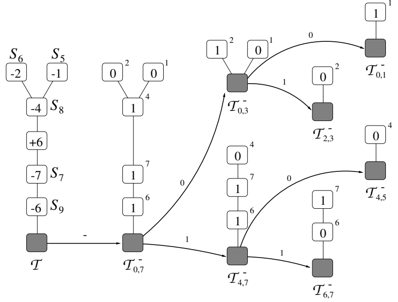
Figure 3.7: Hierarchical binary partition of a labeled ordinal tree for root-to-node path queries, reproduced from Gagie, He, and Navarro [9]. Starting from the root range, each intermediate tree \mathcal{T}_{a,b} is 0/1-labeled by the midpoint of its range. Bold arrows lead to the child trees \mathcal{T}_{a,m} on marker 0 and \mathcal{T}_{m+1,b} on marker 1. The binary alphabet at every level makes each level transition cost O(1) via a single rank or select on the marker sequence.
