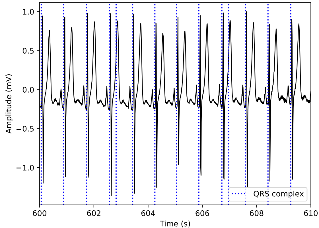
Electrocardiogram: b02
