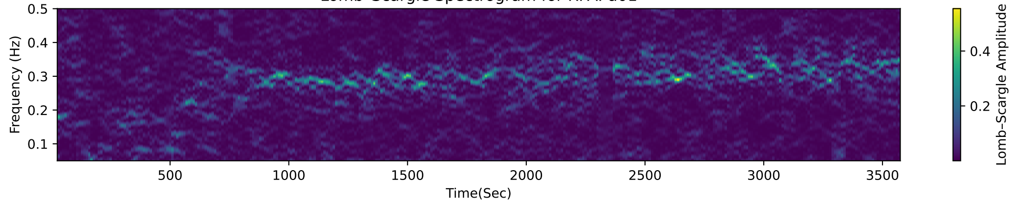
Lomb-Scargle Spectrogram for RPA: a01
