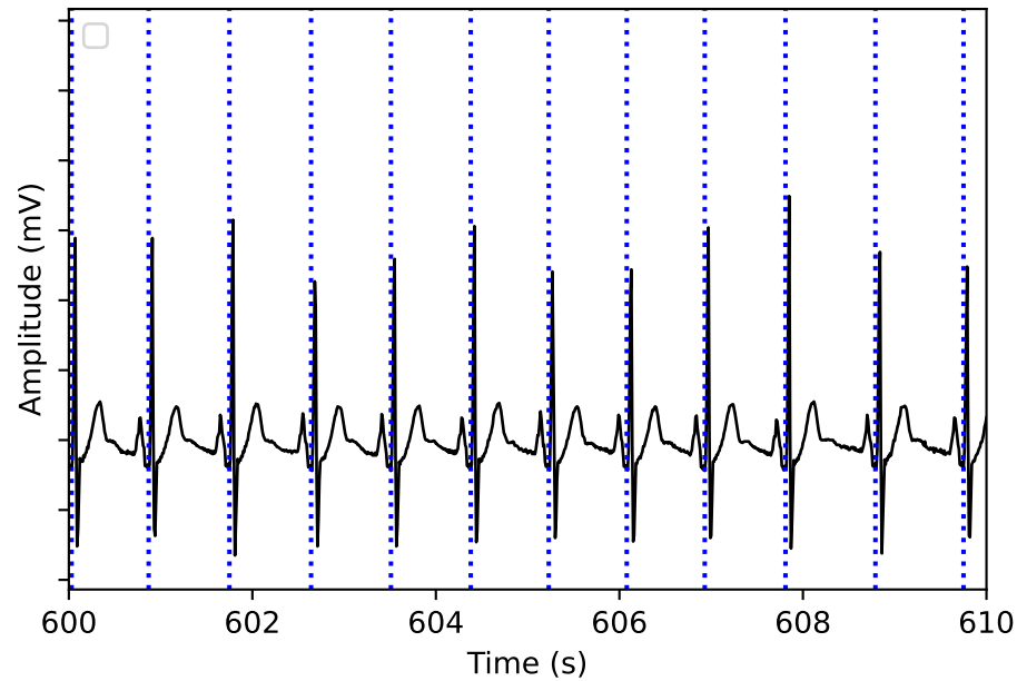
Electrocardiogram: a01
