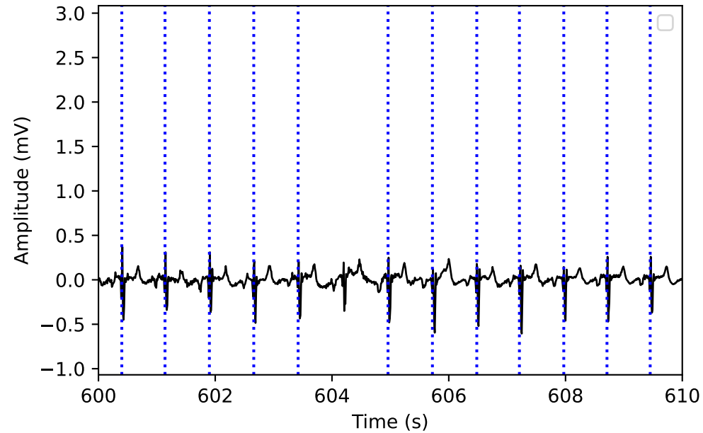
Electrocardiogram: a12
