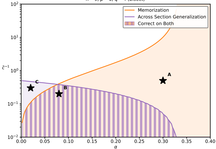
Phase diagram: representational geometry vs. regularization
