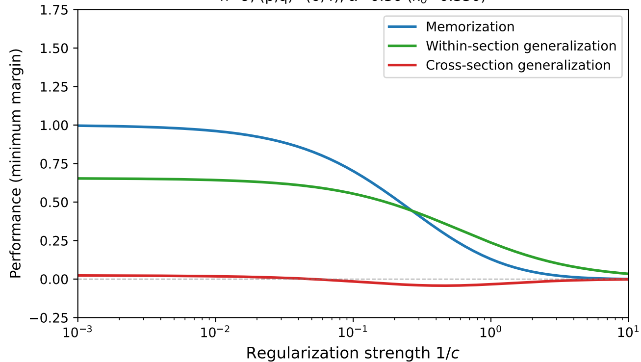
Performance vs. regularization strength n=9 , (p,q)=(6,4) , \alpha=0.30 ( k_o=0.350 )
