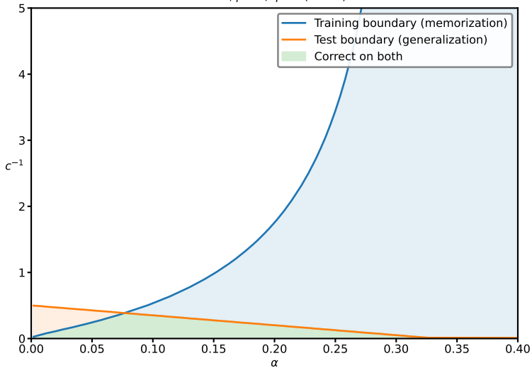
Phase diagram: representational geometry vs. regularization n = 9, p = 6, q = 4 (bisect)
