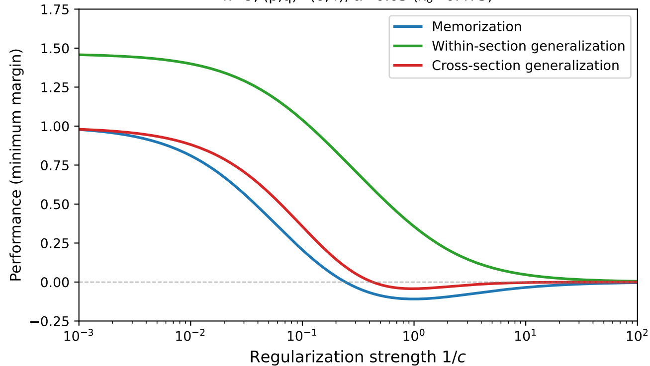
Performance vs. regularization strength n=9 , (p,q)=(6,4) , \alpha=0.05 ( k_o=0.475 )
