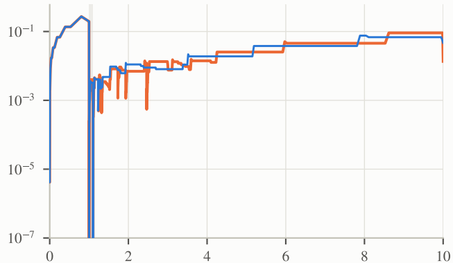
GENROU boundary (knee at operating point, no gates)
