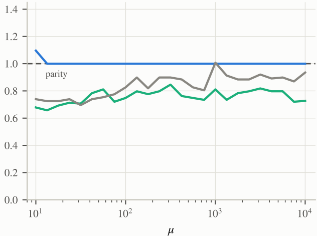
GENROU saturated: accepted h
