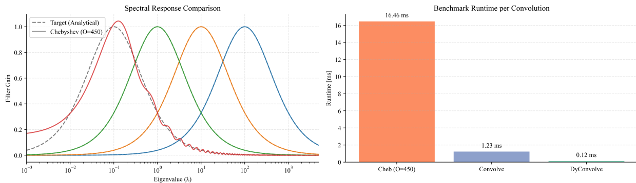
Chebyshev vs. Analytical Timing Comparison Polynomial Order k = 450 | Scales: 4
