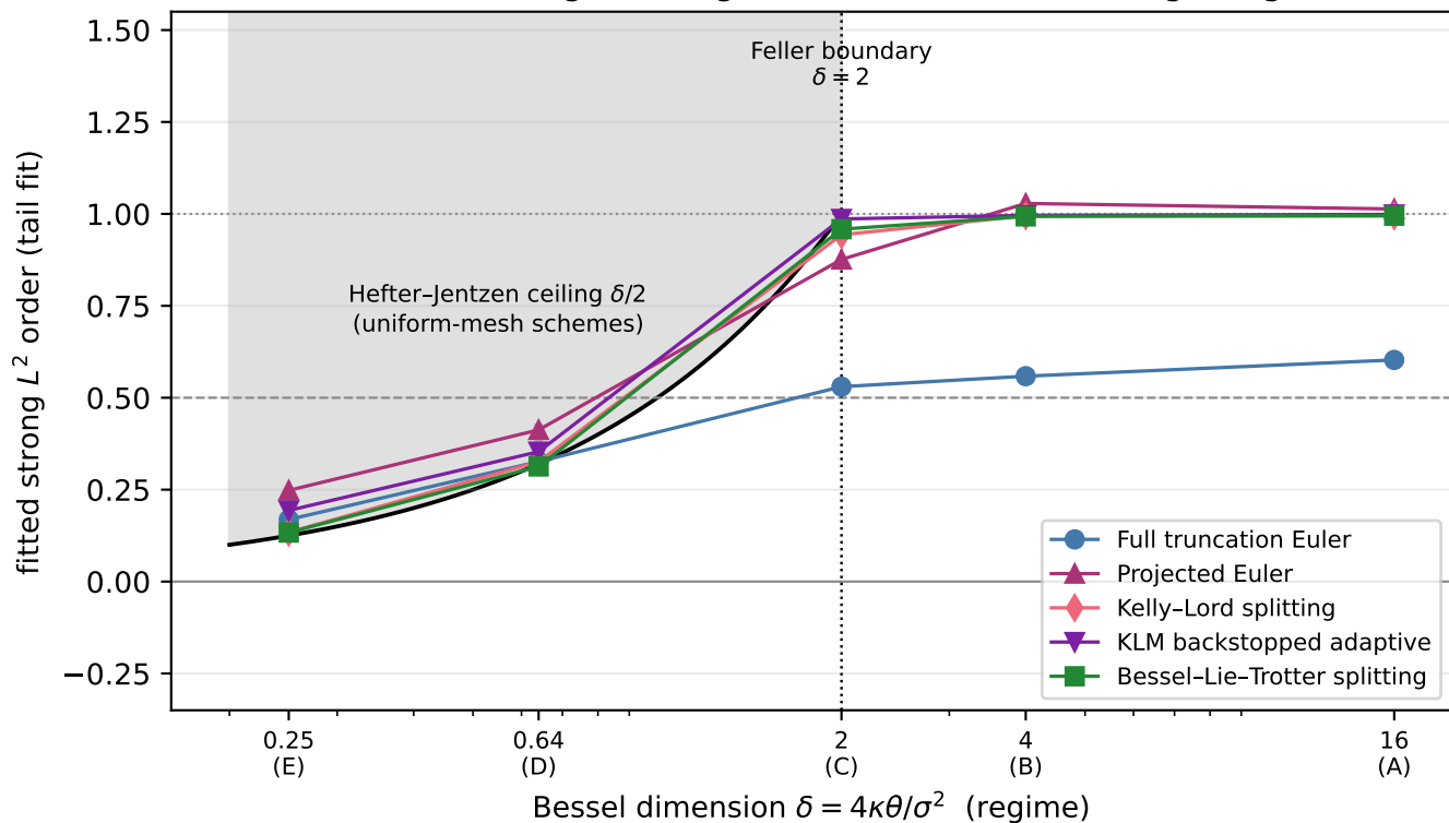
Observed strong convergence order across the regime grid
