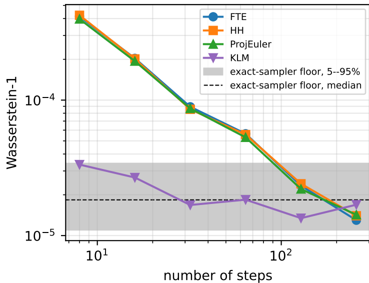
Regime A
