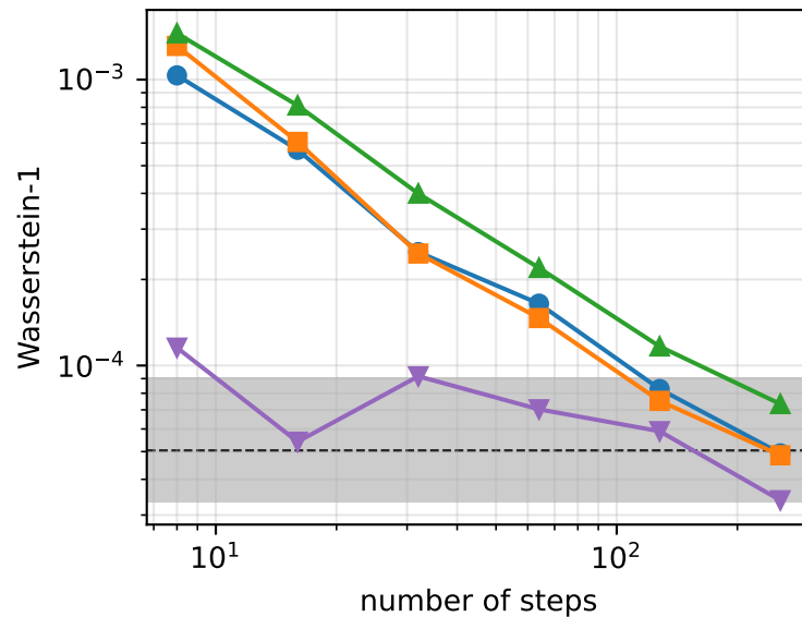
Regime C
